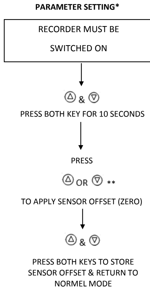
Figure 16- ELECTRICAL CALIBRATION
