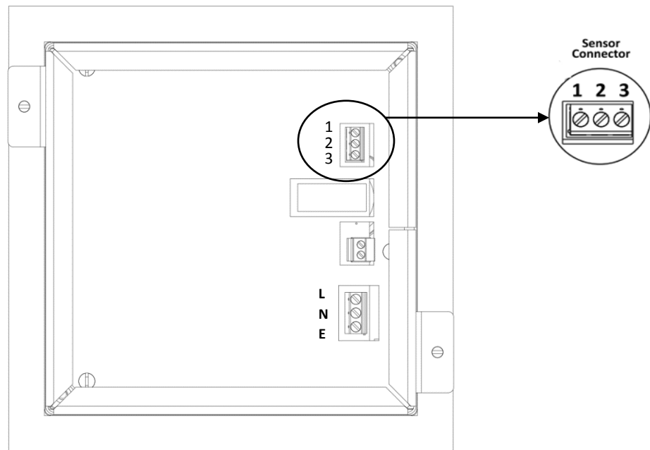
Figure 7- SENSOR WIRING
