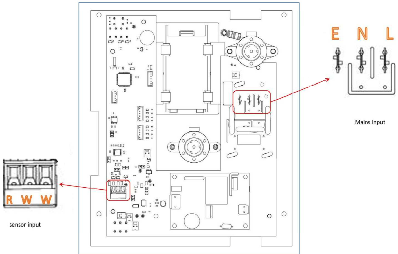
Figure 7 - Sensor and Mains connection
