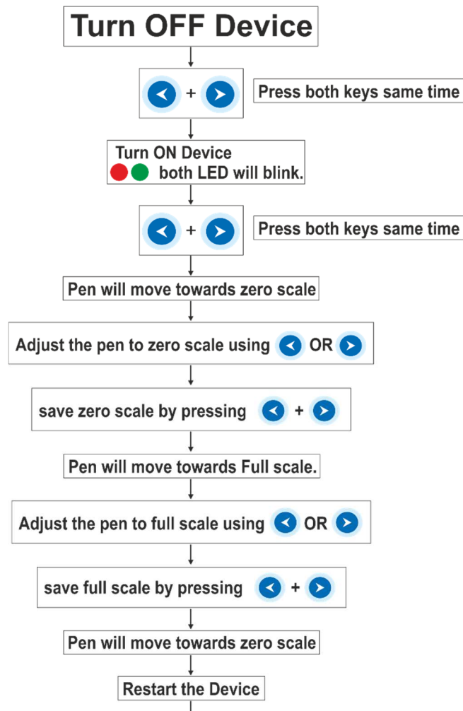
Figure 12 - Mechanical Calibration sequence
