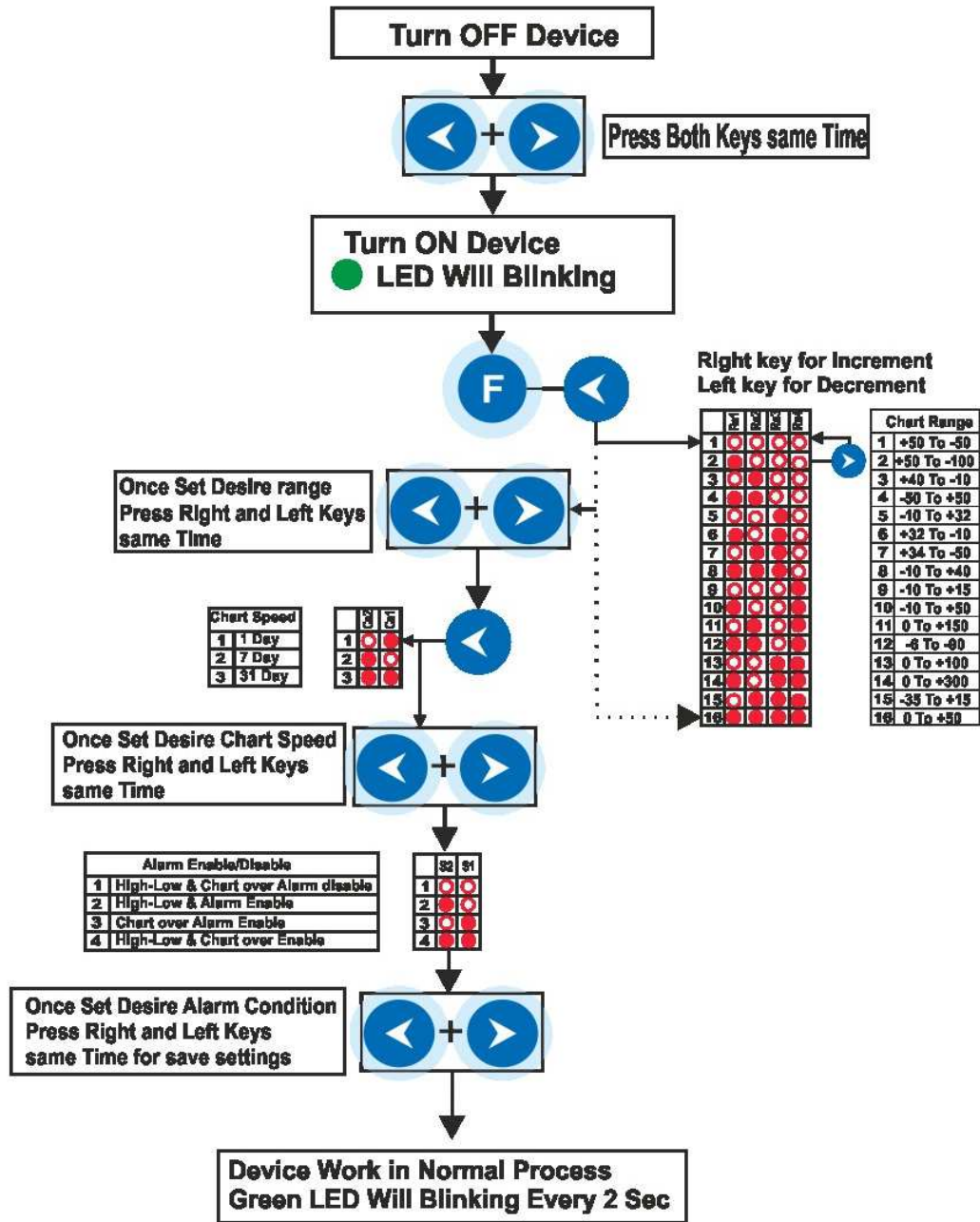
Figure 11 - Chart Parameters settings sequence
