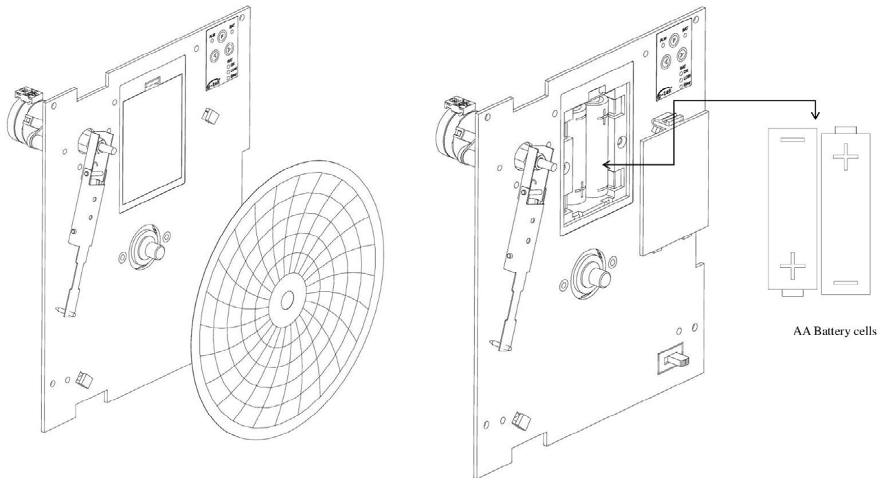
Figure 15 - Battery Replace
