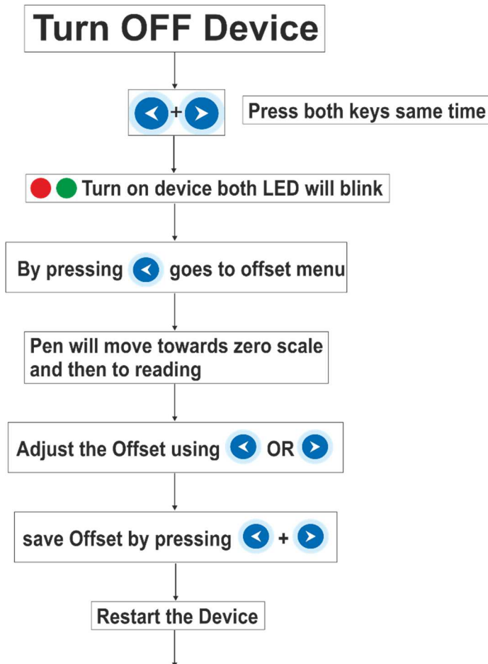
Figure 13 - Offset Settings sequence
