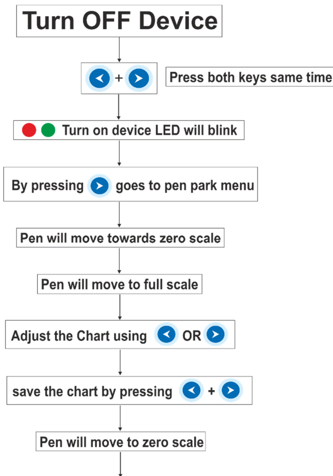
Figure 14 - Pen-Park Function sequence
